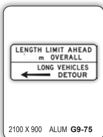
900 X 900 ALUM G9-73A 1200 X 1200 ALUM G9-73B
